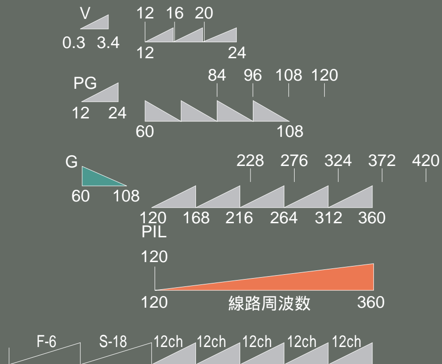
X-60方式の周波数配置( kHz ) Frequency allocation in X-60 system
